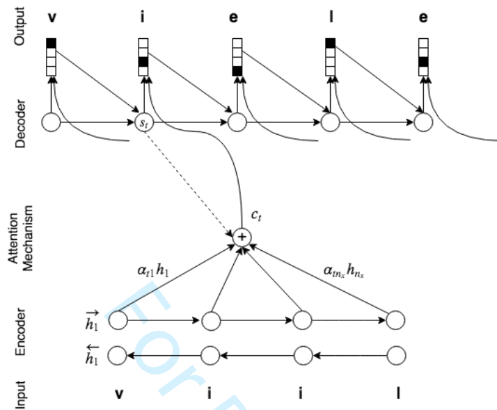
Fig. 1. Basic NMT architecture.
