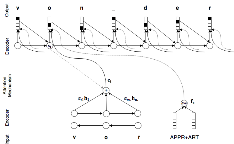
Fig. 2. NMT with POS tags as features.
